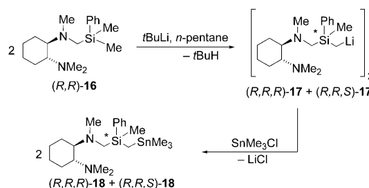
Scheme 7. Asymmetric lithiation of dimethylsilane ( R,R )- 16 and trapping with trimethyltin chloride to afford stannane 18 .
