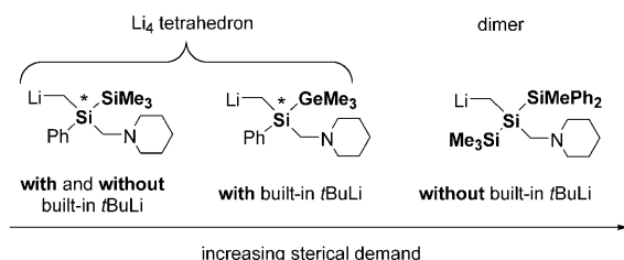
Figure 7. Comparison of the different structural motifs of the lithiated silanes.
